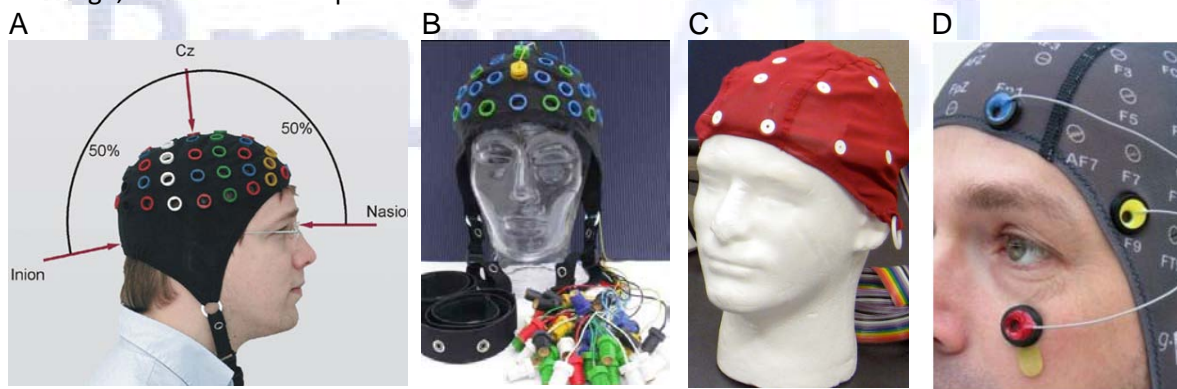
Figure 2: Electrode caps according the 10/20 electrode system
